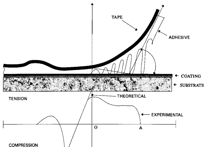
FIG. X1.1 Peel Profile (6)
