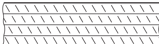
Figure 2 — Example of rib pattern for grade B500A
