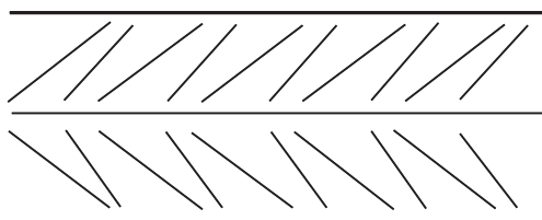
Figure 4 — Example of rib pattern for grade B500C
